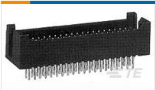
TE Part # 6-534978-5 70 MODII 2PC HDR DR W/HLDWN, ROHS
